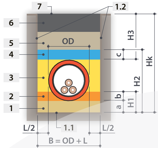
Cross section of the protection pipe trench (according to clause 3, Figure 1, EN 1610 standard)
